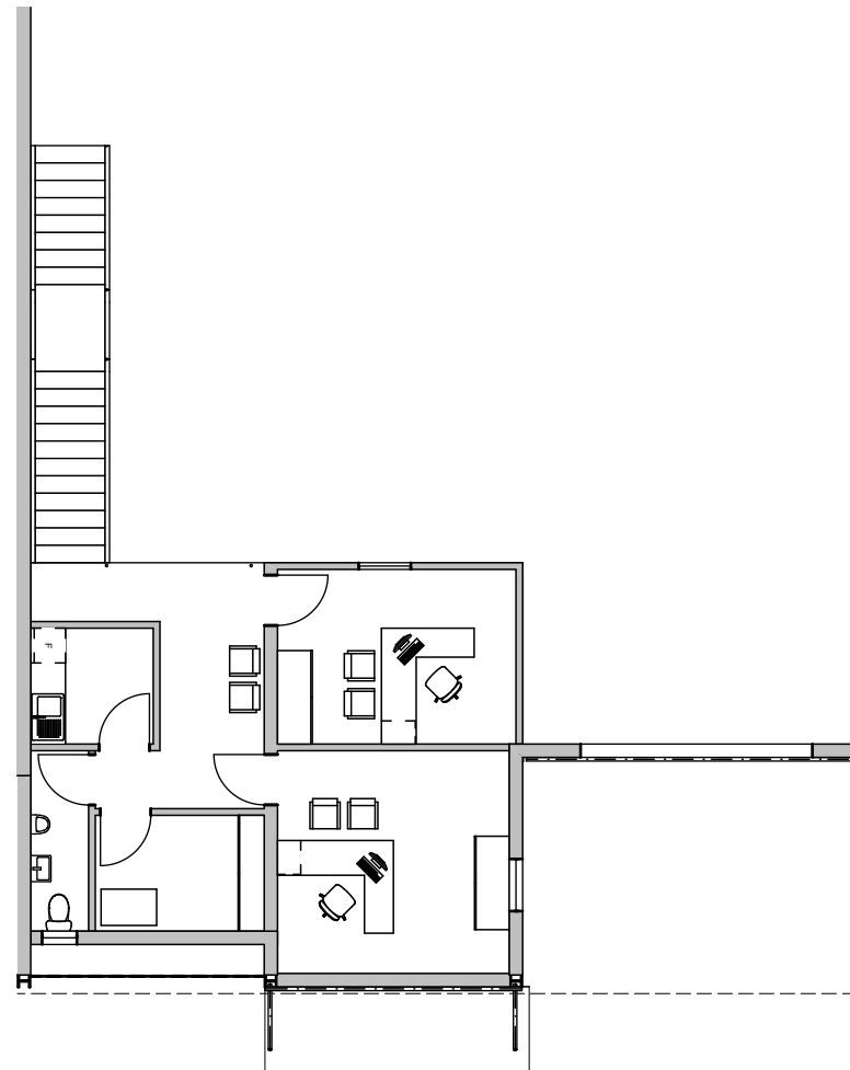
B11 Unit B11 Mezzanine Level:200
